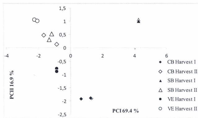
Figure 1. PCA obtained from 18 white wine samples analyzed by GC-FID in two harvest dates, in June (Harvest I) and November (Harvest II) of 2009, for the determination of the higher alcohols. PC1 x PC2 explained 86,3% of the total variability. CB: Chenin blanc; SB: Sauvignon blanc; VE: Verdejo.
