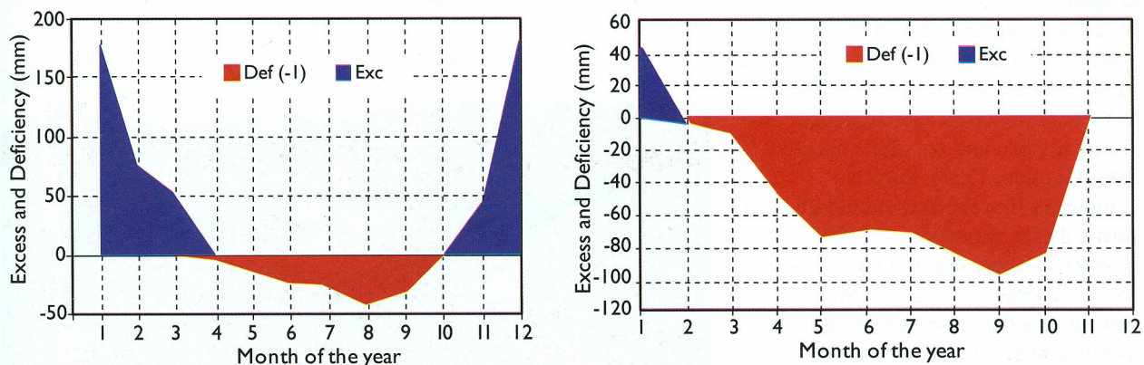
Figure 4. Monthly hydrological soil water balance variation at the specific sites at the Embrapa Maize and Sorghum experimental fields at Sete Lagoas (left), and Janaúba (right), based on climatic time series databases covering 45 years (1960–2005) and 14 years (1977–1990) respectively, and assuming a total soil water availability of 100mm to a depth of 1m.
