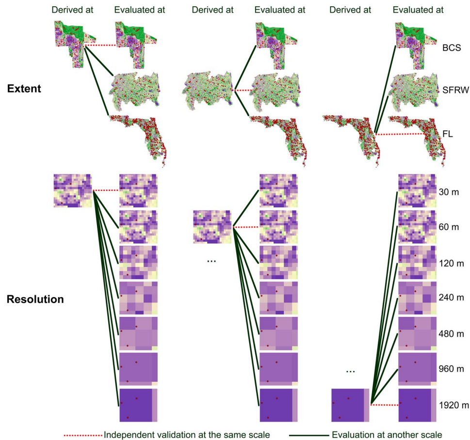
Figure 2. Overview of the framework used to test the influence of the spatial extent and resolution of input data on the stepwise multiple linear regression models of ln-transformed soil total carbon. BCS is the University of Florida Beef Cattle Station, FL is Florida, and SFRW is the Santa Fe River watershed.
