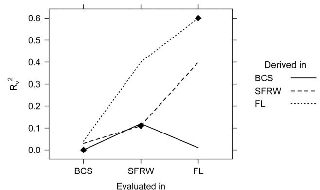
Figure 3. Evaluation of the stepwise multiple linear regression models of ln-transformed soil total carbon among spatial extents. BCS is the University of Florida Beef Cattle Station, FL is Florida, and SFRW is the Santa Fe River watershed. Diamonds indicate validation in the same extent that the model was derived.
