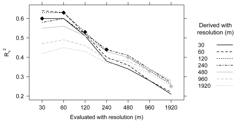
Figure 5. Evaluation of the stepwise multiple linear regression models of ln-transformed soil total carbon among resolutions of input data in Florida. Diamonds indicate validation at the same resolution that the model was derived.
