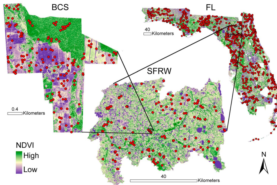
Figure 1. Sampling locations at the three nested study areas (spatial extents). BCS is the University of Florida Beef Cattle Station, FL is Florida, and SFRW is the Santa Fe River watershed. Normalized difference vegetation index (NDVI) is shown in the background.
