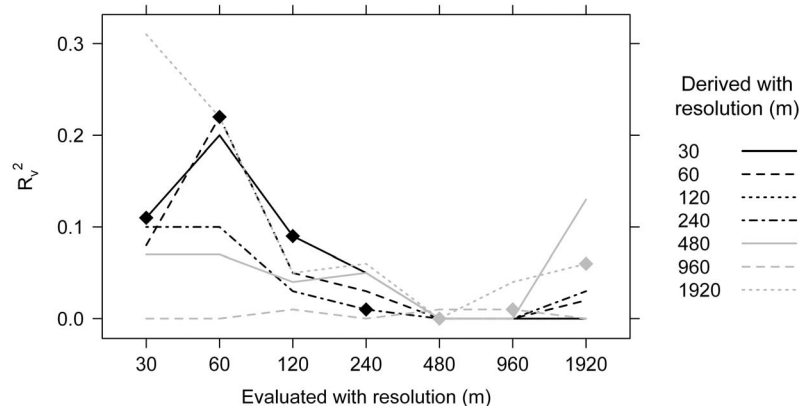
Figure 6. Evaluation of the stepwise multiple linear regression models of ln-transformed soil total carbon among resolutions of input data in the Santa Fe River watershed. Diamonds indicate validation at the same resolution that the model was derived.
