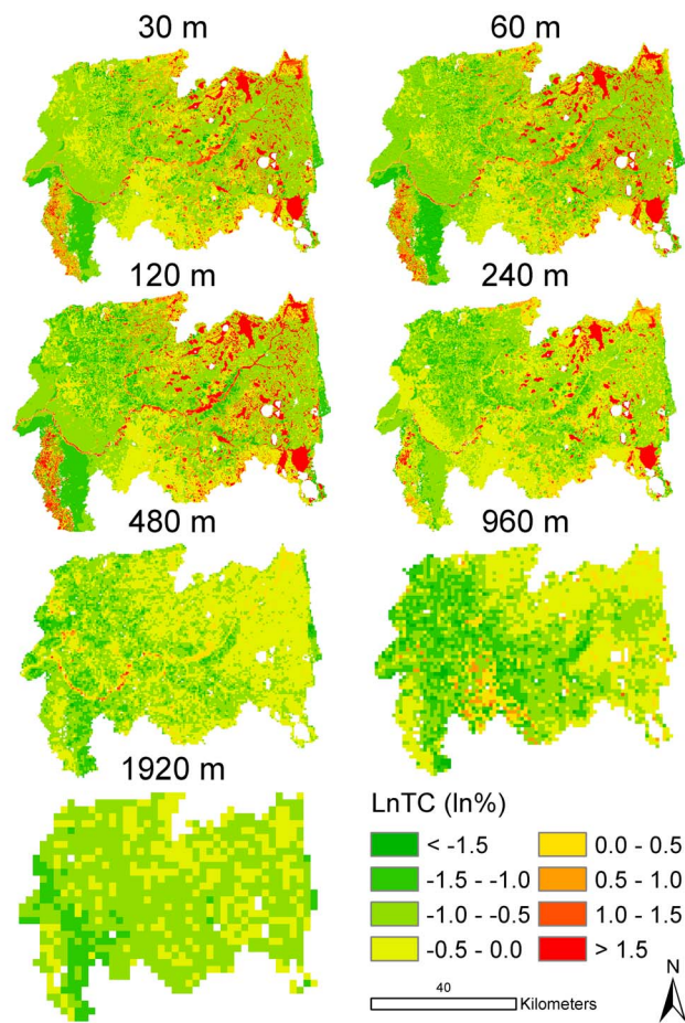
Figure 4. Estimated maps of ln-transformed soil total carbon (LnTC) from the stepwise multiple linear regression models derived for seven resolutions of input data, respectively, in the Santa Fe River watershed.
