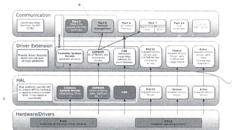
Fig. 3. Structure view of IsoAgLib modular design. Source: IsoAgLib (2012).
