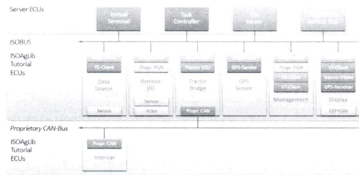
Fig. 4. ISO 11783 Network with IsoAgLib. Source: IsoAgLib (2012).
