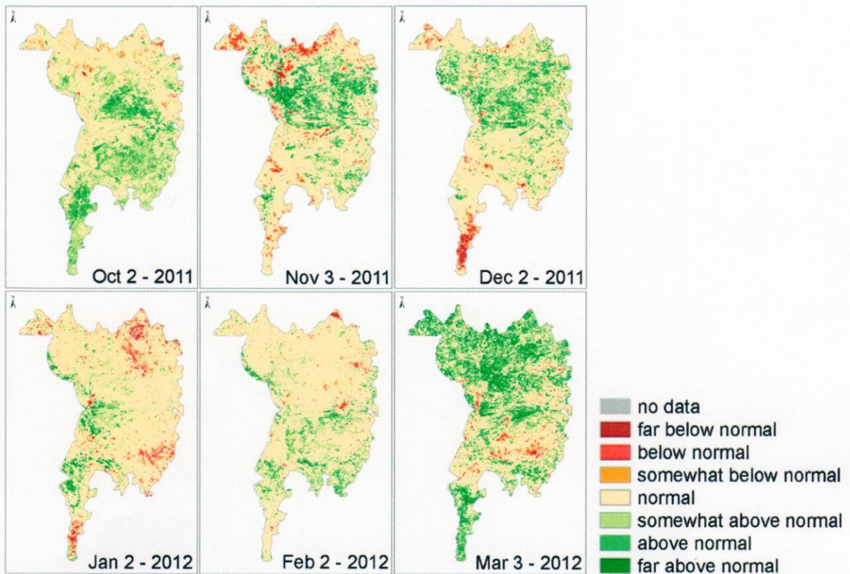
Figure 3 - Spatial distribution of the Standardized Vegetation Index in the rainy season, from October 2011 to March 2012
