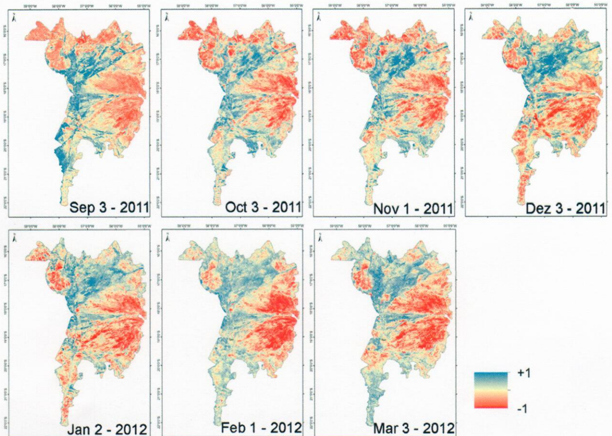
Figure 5 - Spatial distribution of the NDWI index from September 2011 to March 2012
