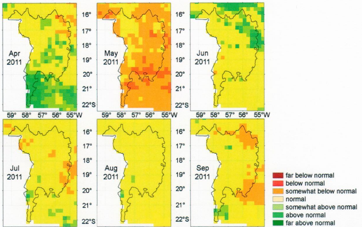
Figure 4a - Spatial distribution of the Standardized Rainfall Index (SRI) obtained from the TRMM sensor, from April 2011 to March 2012 (dry season)
