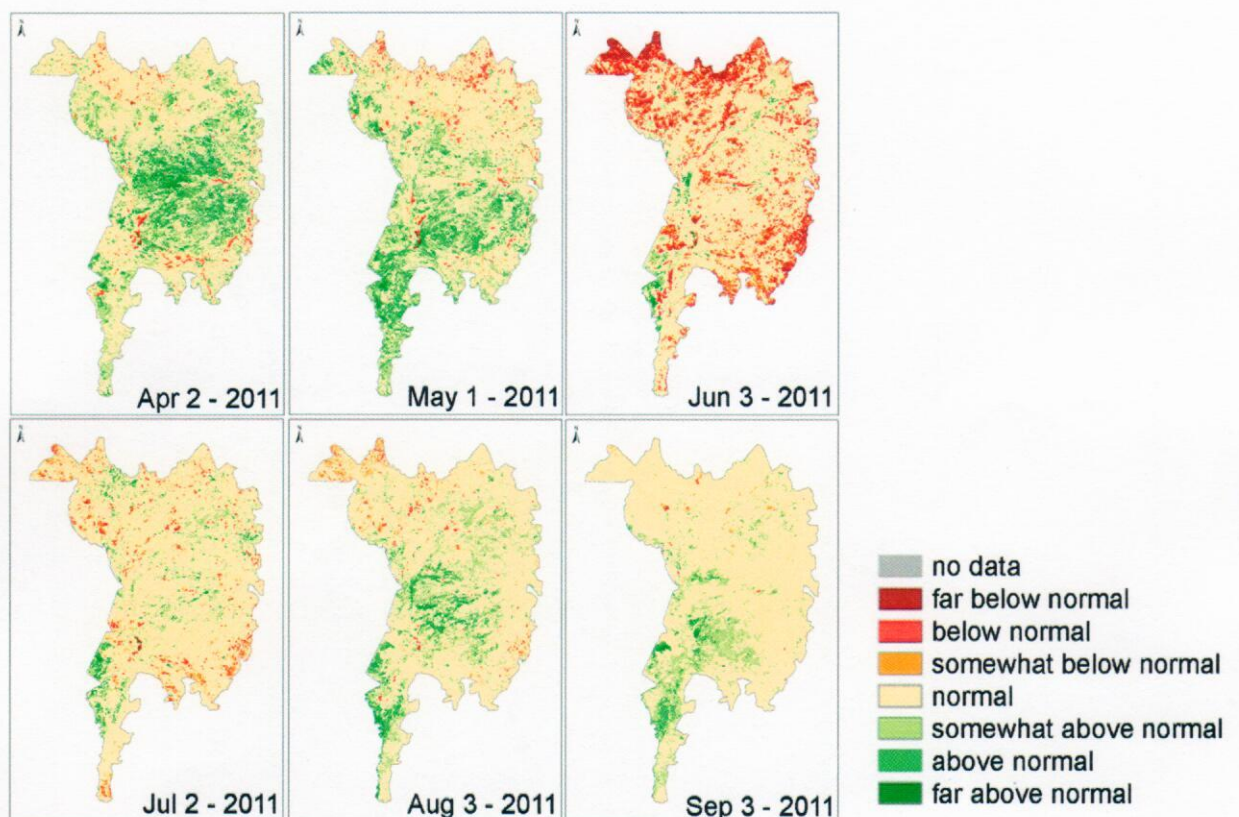
Figure 2 - Spatial distribution of the Standardized Vegetation Index in the dry season, from April to September 2011
